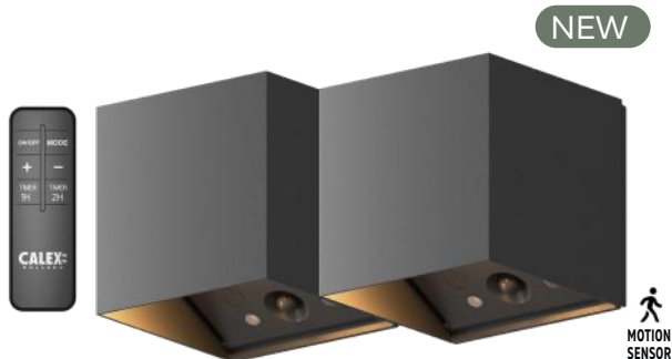
Outdoor Rechargeable Falerna Wall Lamp Black With Motion Sensor (2 pack) Art. # 4301004300 EAN 8712879163862 2700K, 70 Lumen, IP44 incl. USB-C charging cable H:88 x W:88 x D:85 mm
