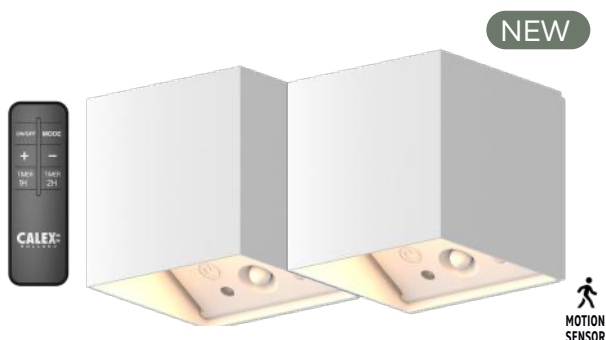
Outdoor Rechargeable Falerna Wall Lamp White With Motion Sensor (2 pack) Art. # 4301005400 EAN 8712879165552 2700K, 70 Lumen, IP44 incl. USB-C charging cable H:88 x W:88 x D:85 mm
