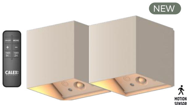
Outdoor Rechargeable Falerna Wall Lamp Sand With Motion Sensor (2 pack) Art. # 4301005500 EAN 8712879165569 2700K, 70 Lumen, IP44 incl. USB-C charging cable H:88 x W:88 x D:85 mm
